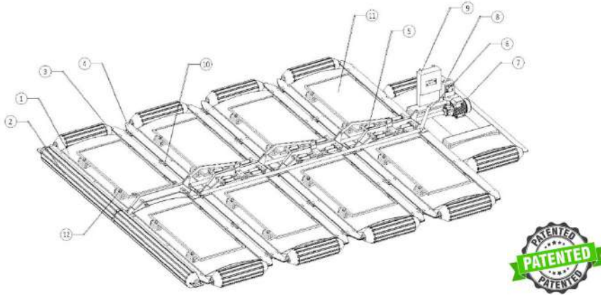
MODULAR FLOATING STRUCTURE FOR FLOATING SOLAR PHOTOVOLTAIC AND FLOATING WAVE HYBRID POWER PLANTS
